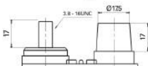
Positive Terminal
