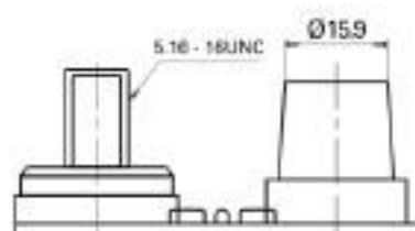
Negative Terminal
